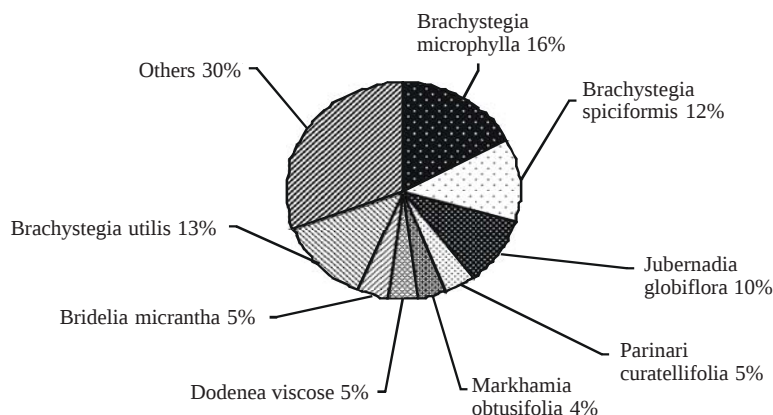
Fig. 4. Distribution of regenerant species in BFR (Number of species = 48)
